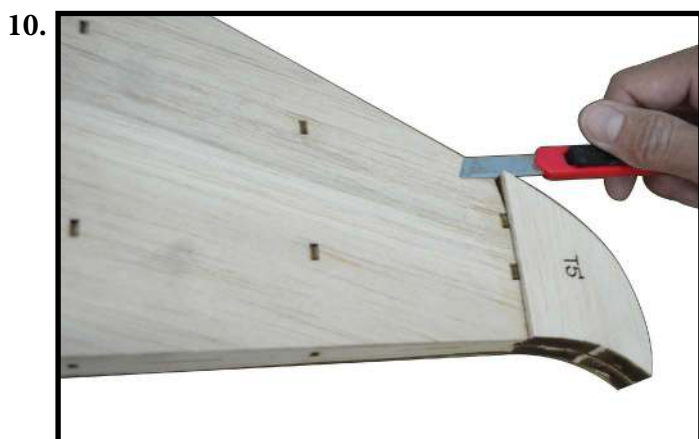
- Use a cutter to sharpen the T5' for flattening surface of rudder.
